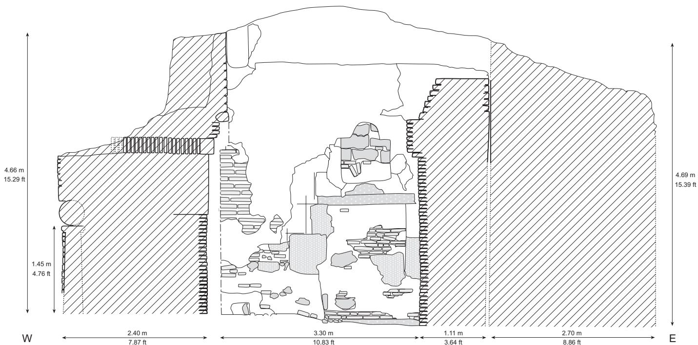
East-West Section, View of North Wall
